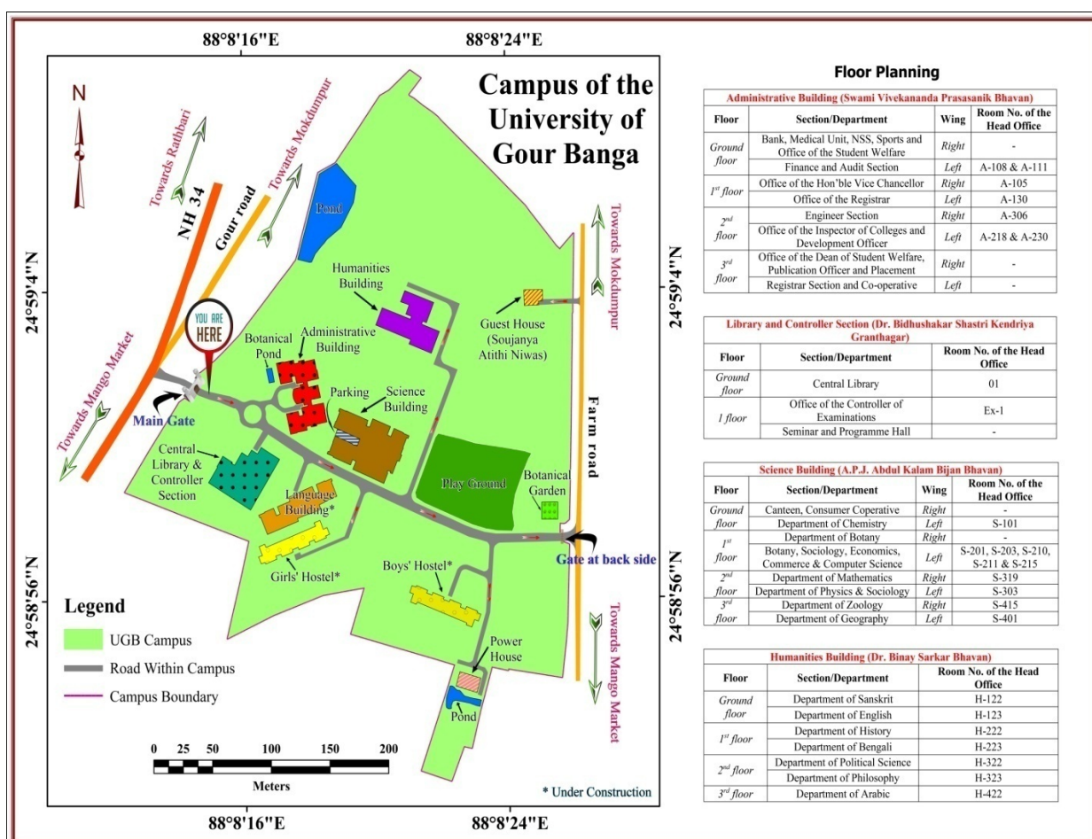
UGB Campus built areas (Academic. Administrative departments, Hostels, Guest house, play grounds, roads)
